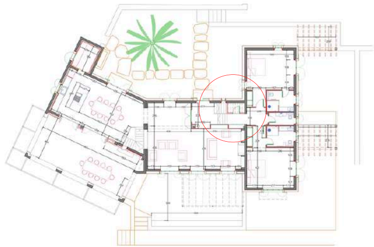
GROUND FLOOR CAN PAREIRA II, DISTRICT OF SANTANYI, POL. 10 PARCEL 1125, E. 1/100 (A3)
